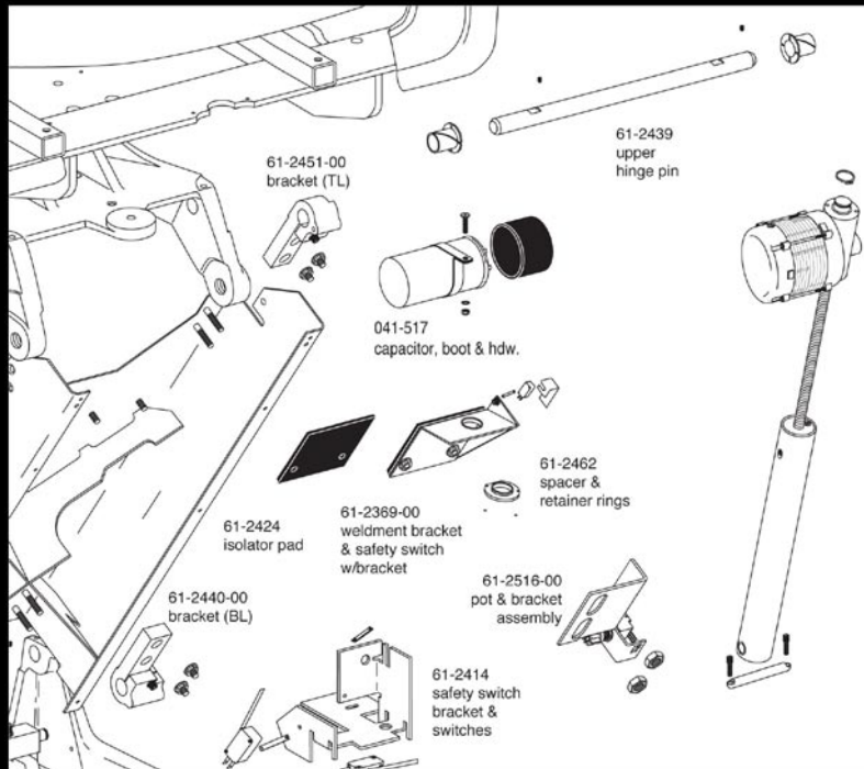
Product Technical Illustration / Adec Manufacturing
